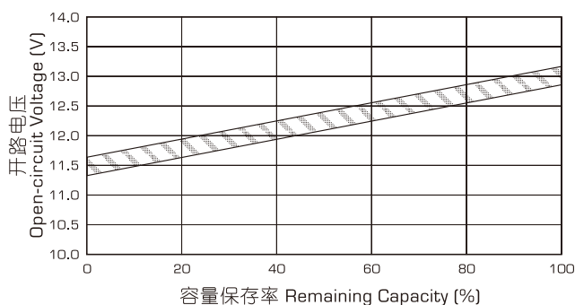
Open Voltage-remaining Capacity
