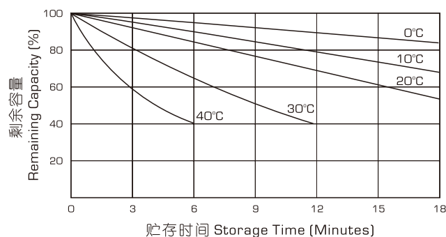
Self discharging characteristics
