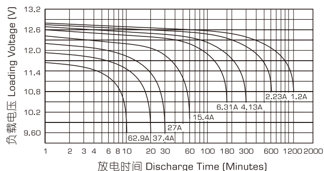
Discharge characteristics
