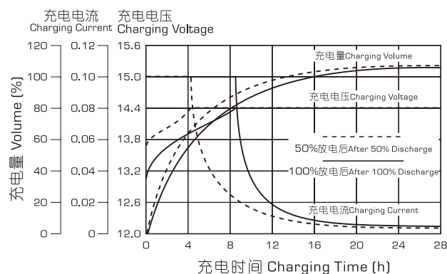
Cycle use charging characteristics
